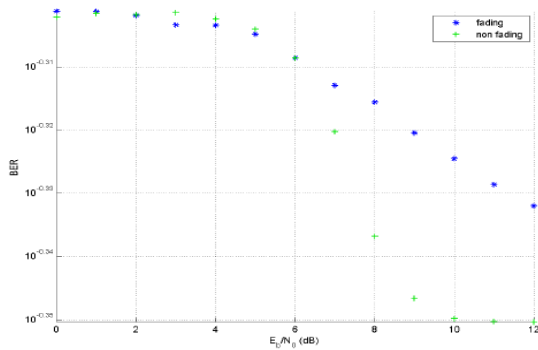
Fig.5: Effect on fading and Non Fading Channels
