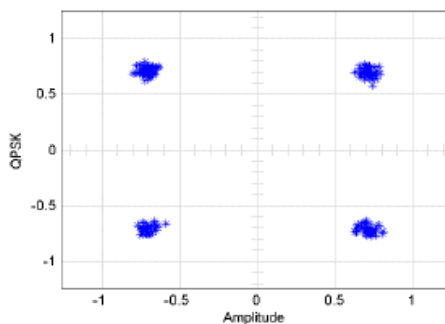
Fig.7: Constellation when SNR=20
