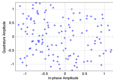
Fig.6: Constellation Diagram at SNR=1
