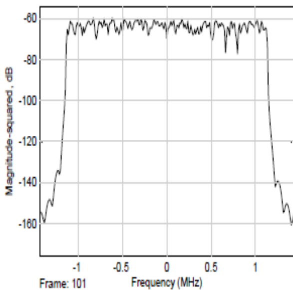
Fig:3: OFDM Signal in Frequency Domain
