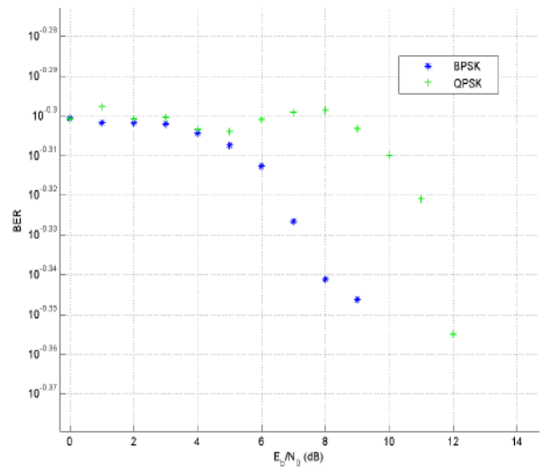
Fig:4: Comparison of Different Modulation Schemes
