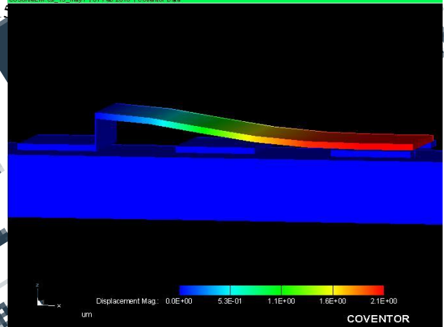
Fig1.2 : Variable Voltage Deflection (3D).
