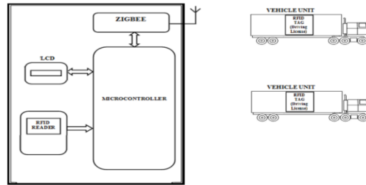
1.4 Handheld Device
