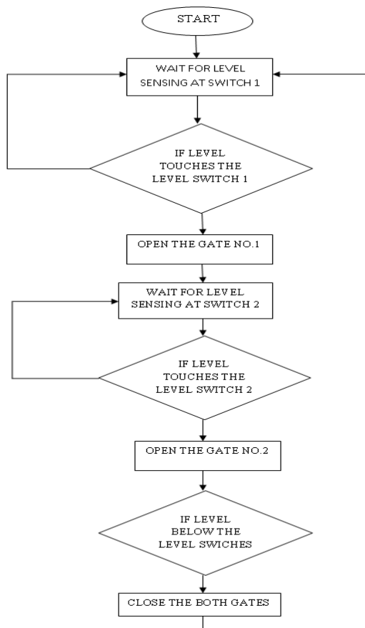
Fig.4 flow chart of proposed control process
