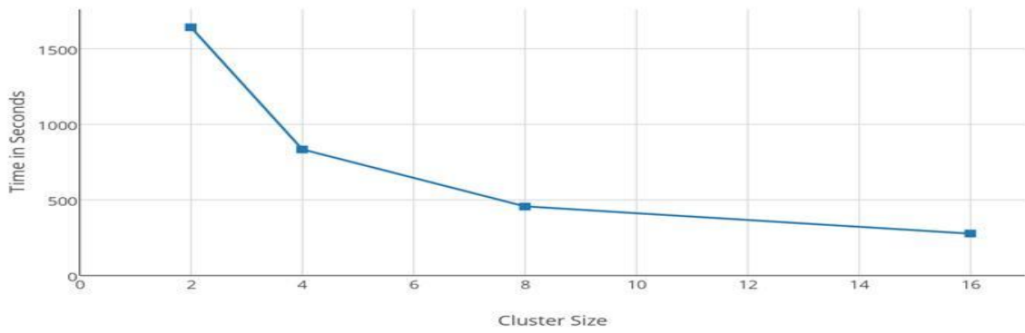
Fig 3 Performance on Multiple Clusters
