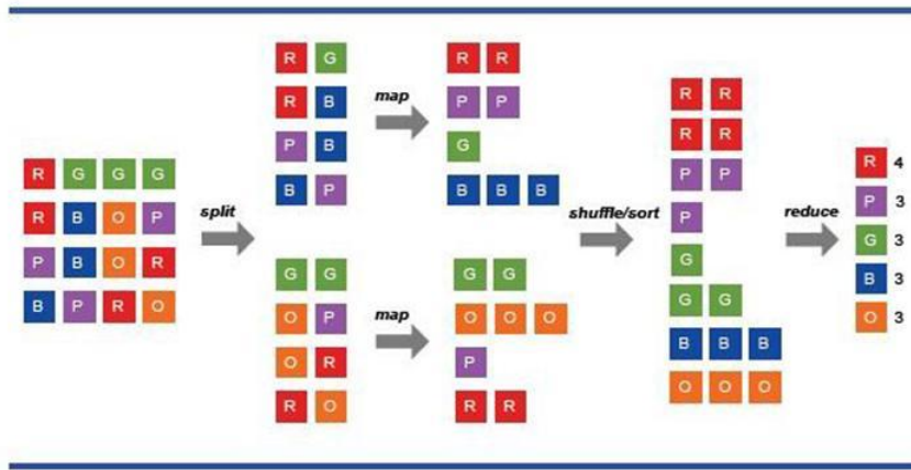
Fig 1 [5] MapReduce Example
