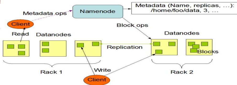
HDFS Architecture
